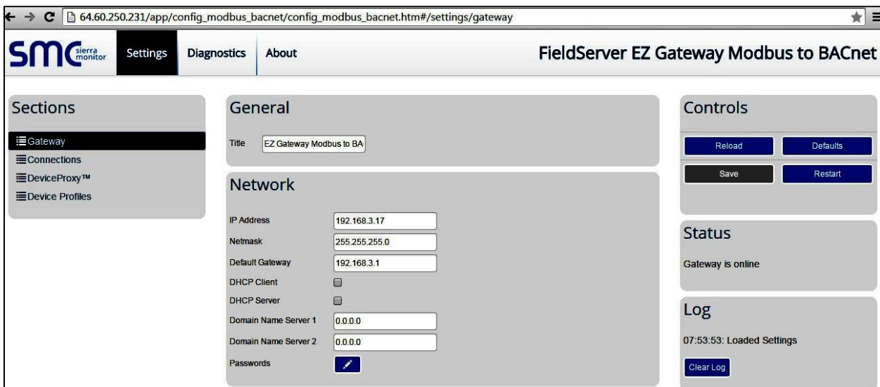
Figure 5: Landing Page
